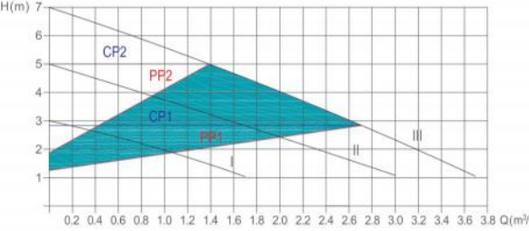
EBV25/7
