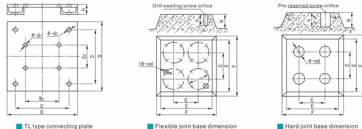
TL type connecting plate
