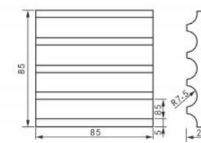
SD type vibration cushion Dimensions
