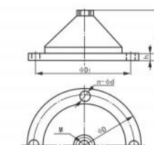
JD type vibration isolator mounting dimensions
