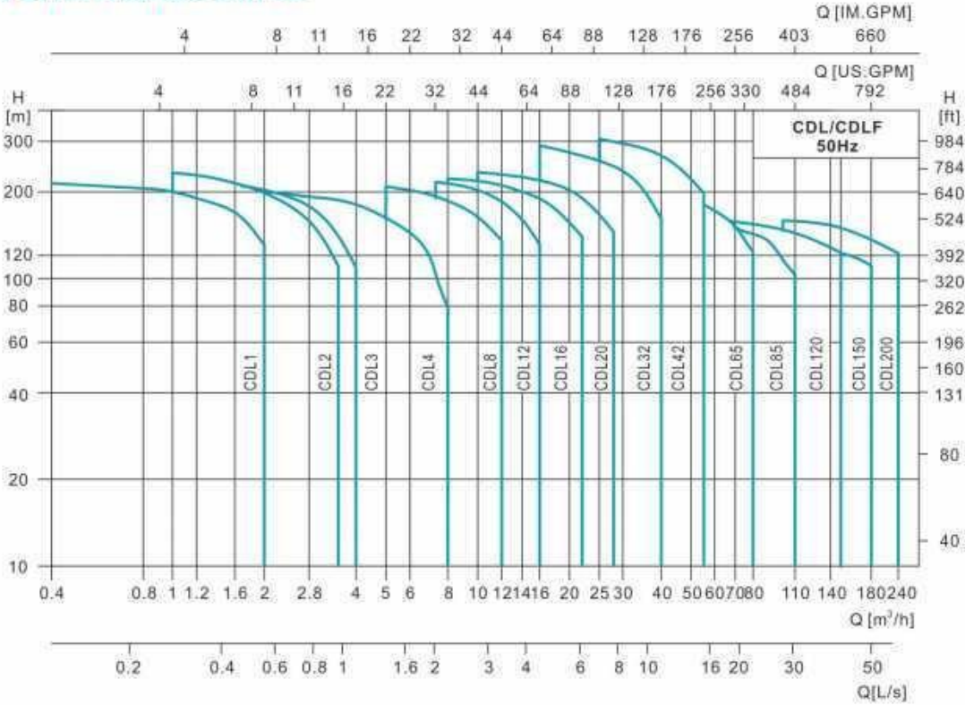
Performance Curve
